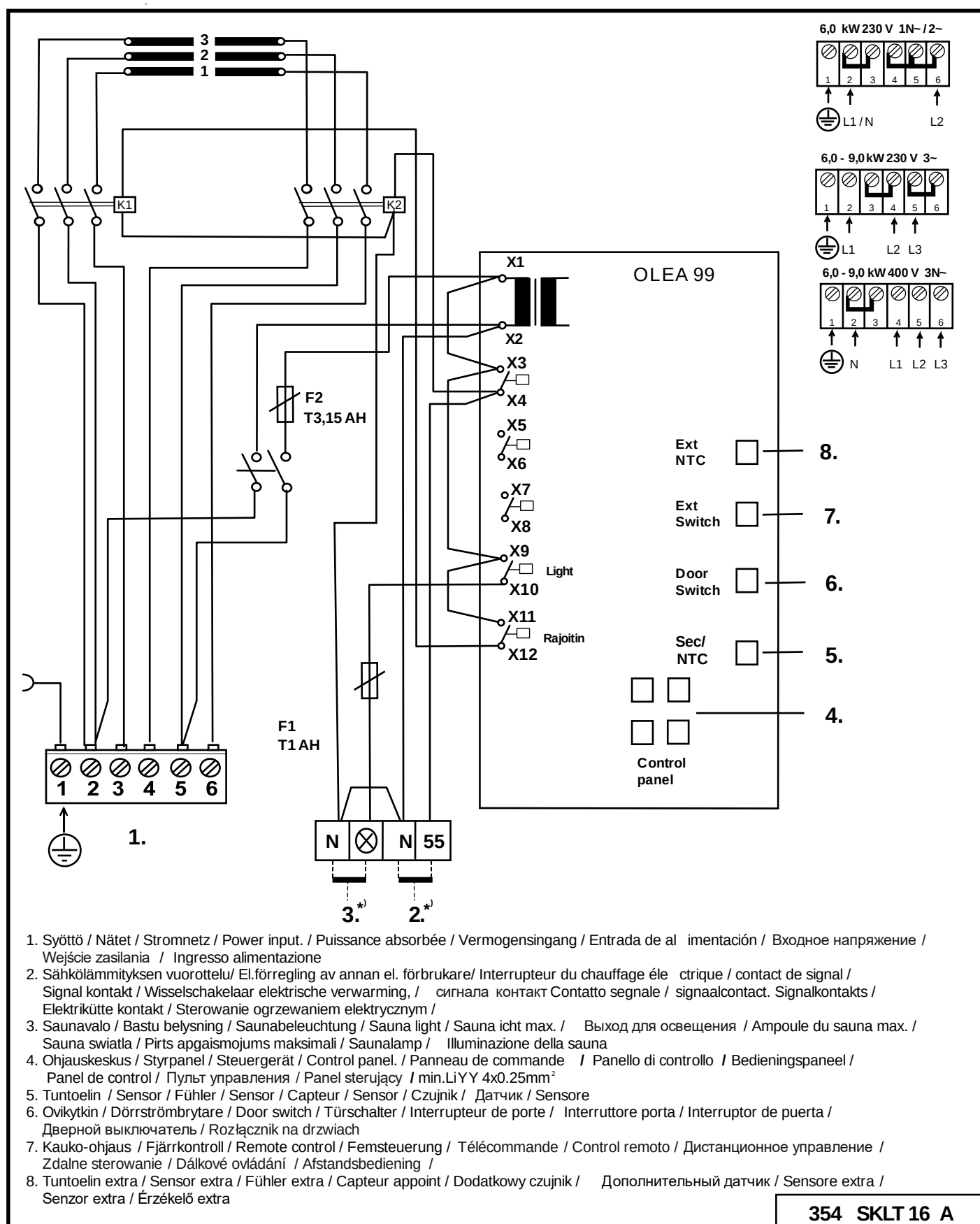
Figure 6. Wiring diagram
