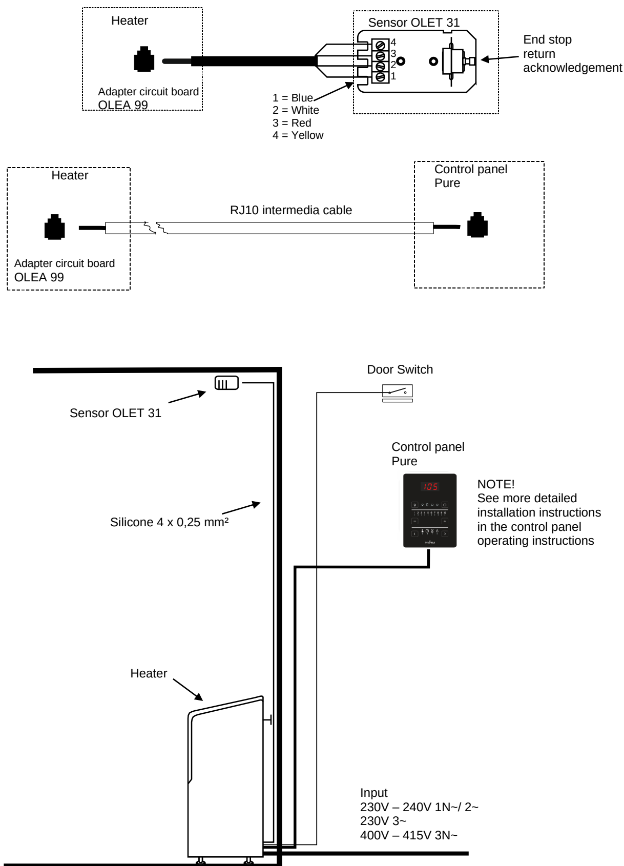
Figure 9 Principle image
