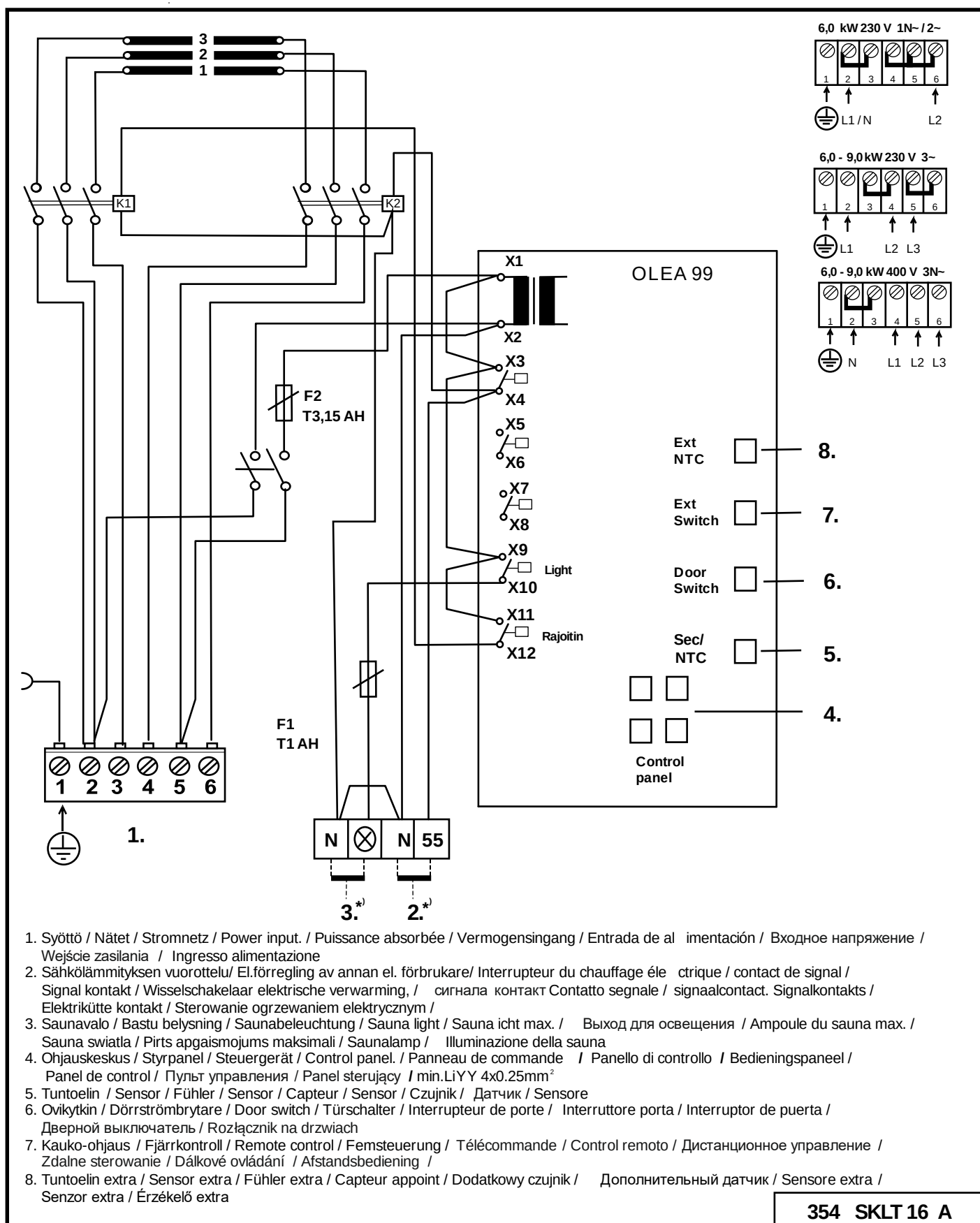
Figure 6. Schéma de raccordement
